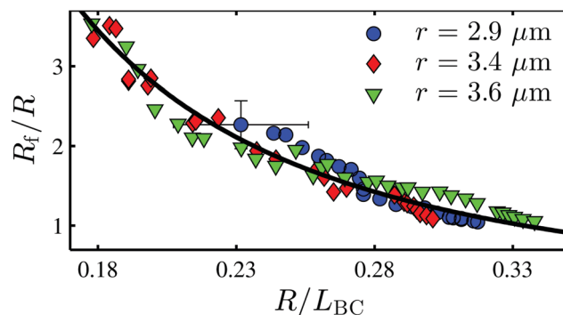
Fig. 3 Central radius of curvature of the fiber normalized by the droplet radius, as a function of the droplet radius normalized by the bending elastocapillary length. One representative set of error bars is shown. The vertical error is dominated by the determination of R_f . The horizontal error bars are the same as in Fig. 2. The solid curve corresponds to the best fit to eqn (3).
